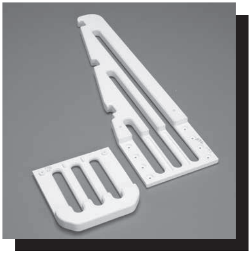
A Lay the Anti-Swim Barrier (M) and its Extension (N) on a flat surface.
