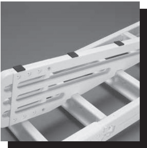
D Evenly space the foam adhesive pads to the Barrier.
