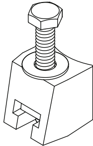
Uses Wedge Assembly PW-P
