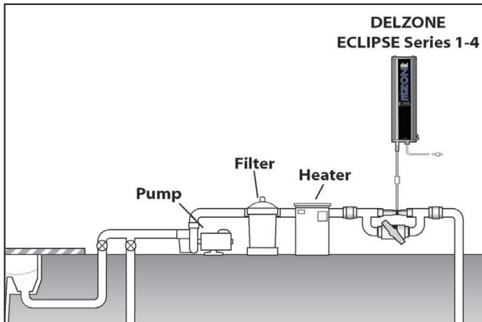
Figure 2 DEL Adjustable Injector Manifold Mounting Location
