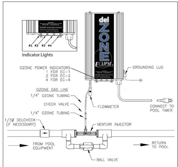
Figure 3 Installation Diagram
