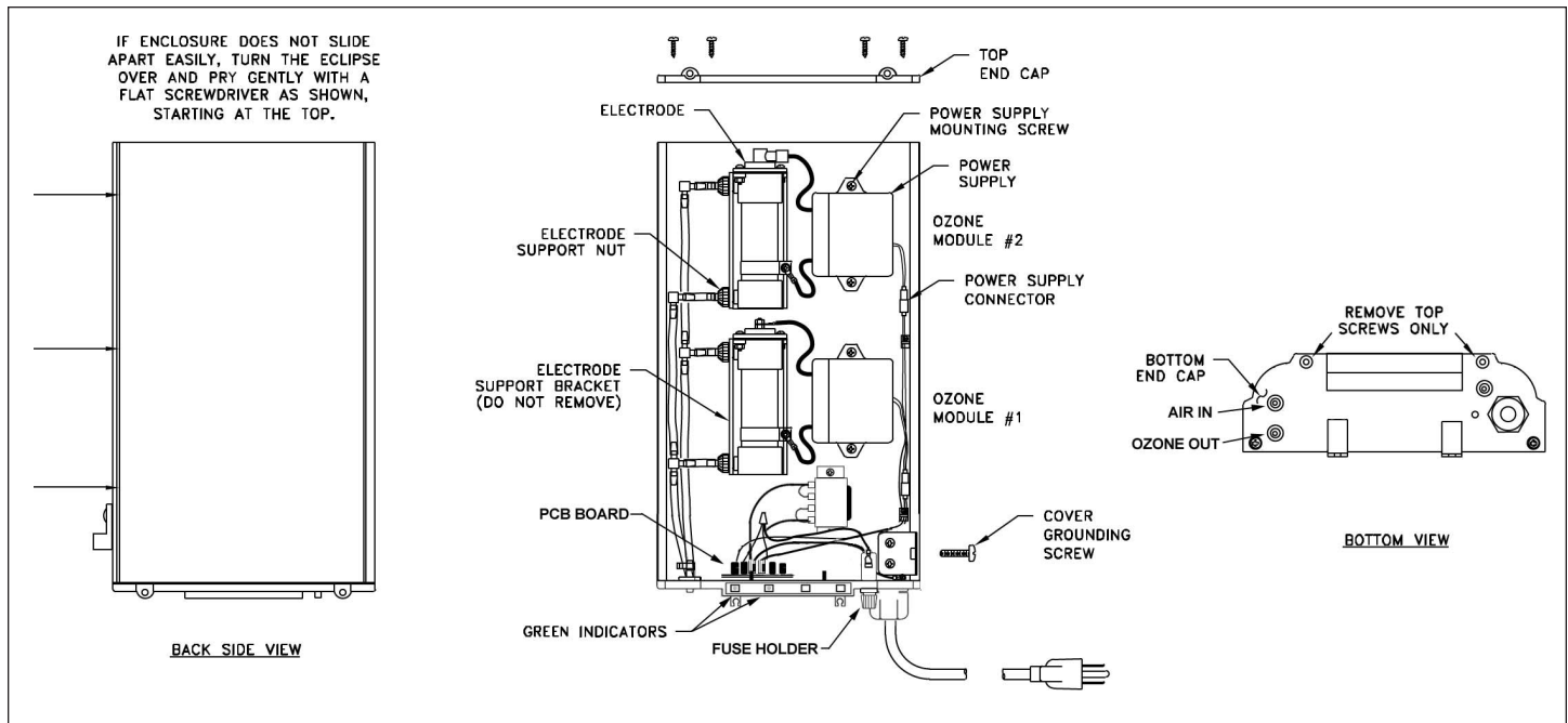
Figure 4 Component Locations (DELZONE® Eclipse-2 Shown)
